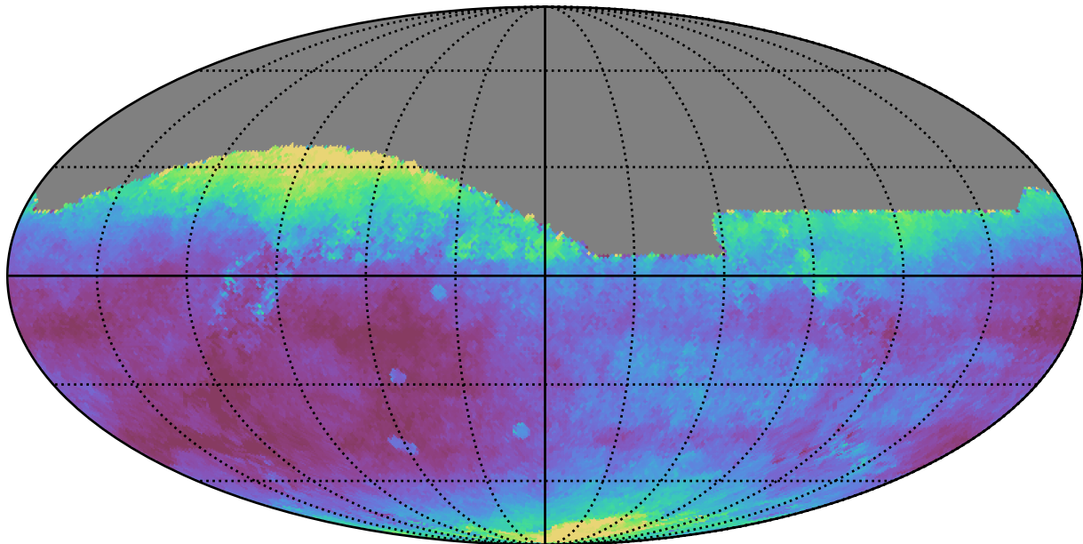
too_elab_r32_d3_griz_v3.4_10yrs All sky r band: Median seeingEff
