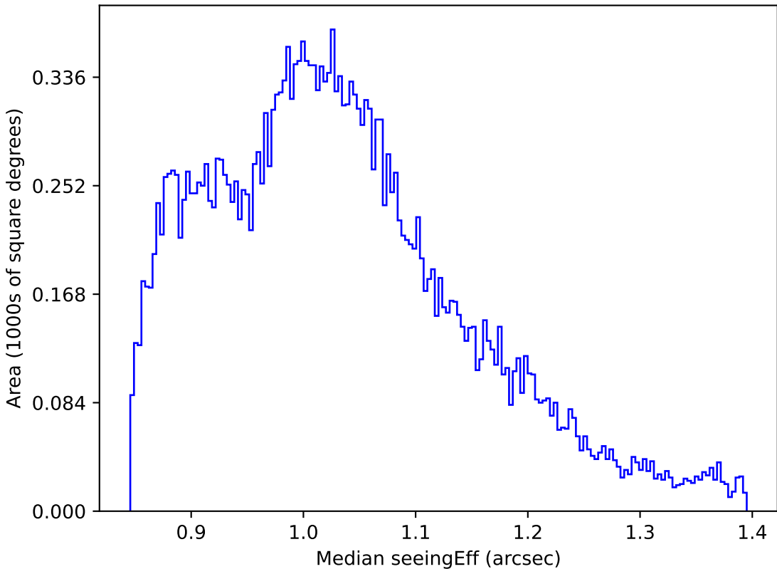
too_elab_r32_d3_griz_v3.4_10yrs All sky i band: Median seeingEff
