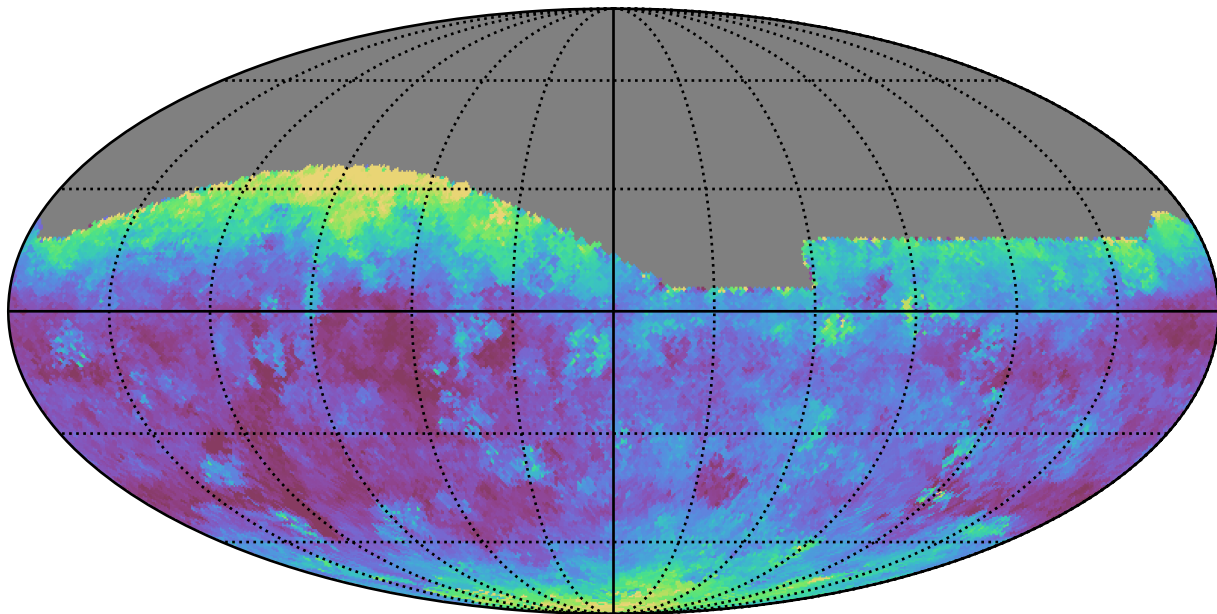
too_elab_r32_d3_griz_v3.4_10yrs All sky g band: Median seeingEff
