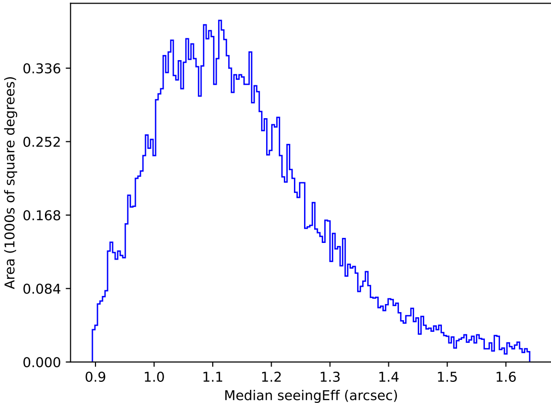
too_elab_r32_d3_griz_v3.4_10yrs All sky g band: Median seeingEff
