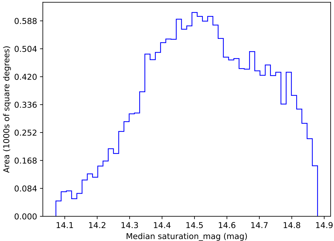
too_elab_r32_d3_griz_v3.4_10yrs WFD i band: Median saturation_mag
