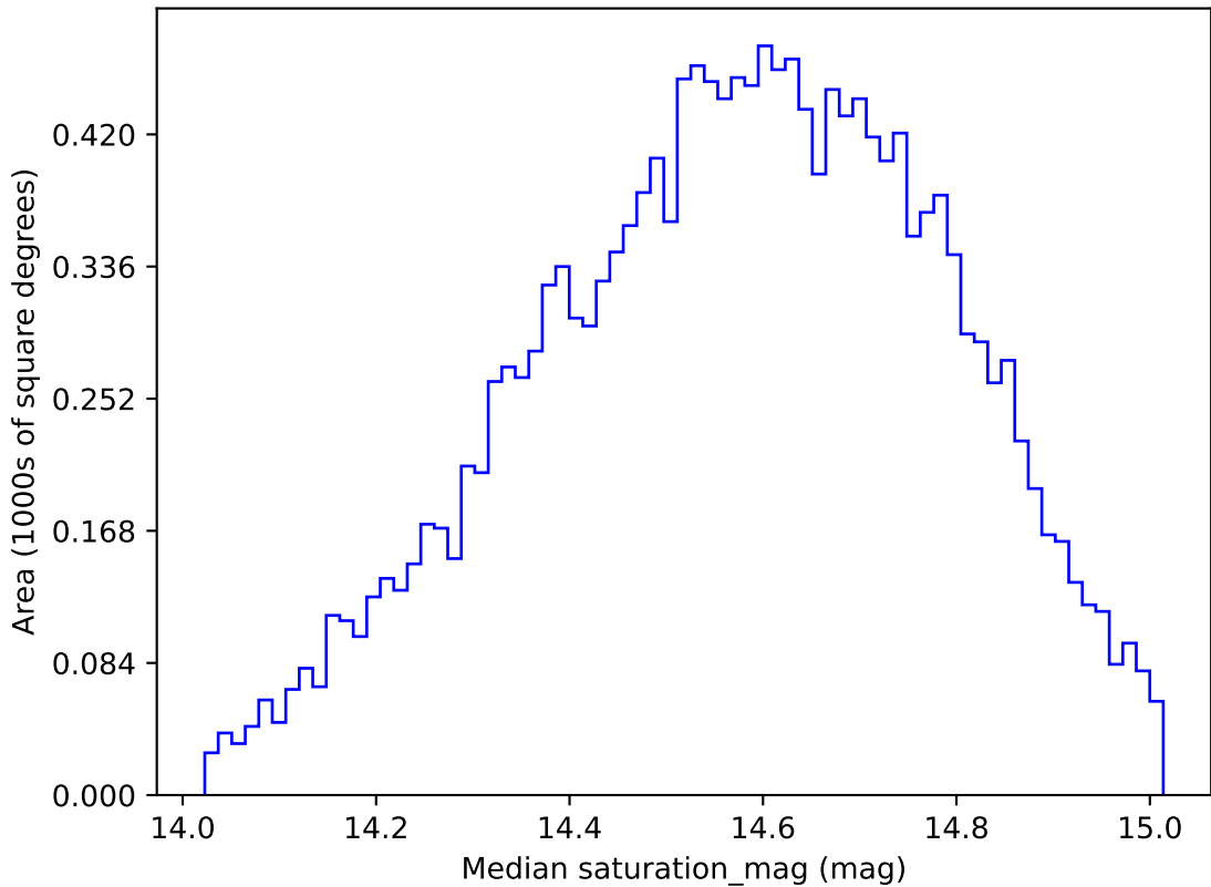
too_elab_r32_d3_griz_v3.4_10yrs WFD g band: Median saturation_mag
