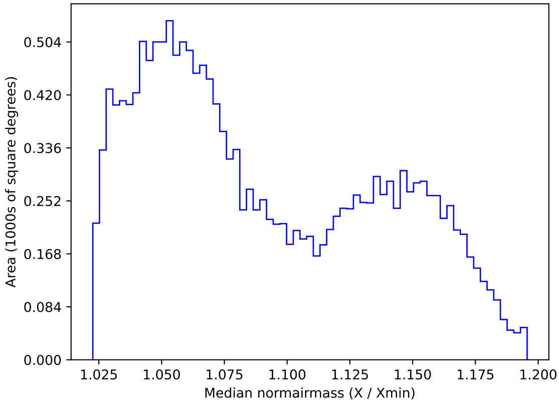
too_elab_r32_d3_griz_v3.4_10yrs WFD z band: Median normairmass
