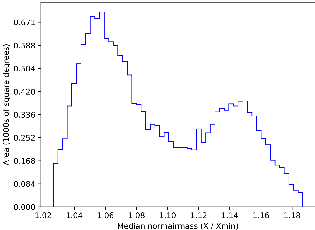
too_elab_r32_d3_griz_v3.4_10yrs WFD y band: Median normairmass
