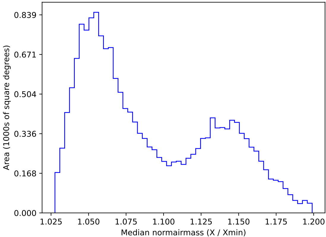
too_elab_r32_d3_griz_v3.4_10yrs WFD y band: Median normairmass
