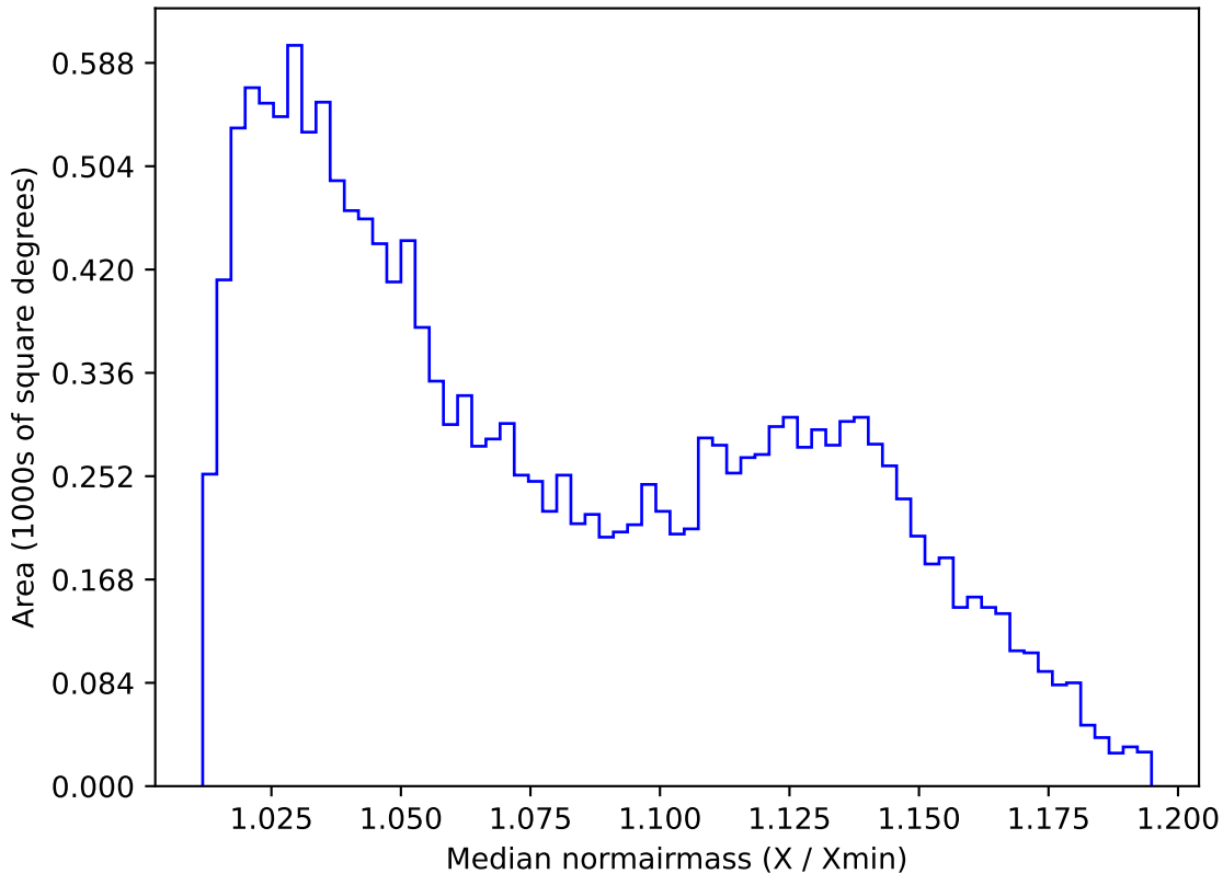
too_elab_r32_d3_griz_v3.4_10yrs WFD u band: Median normairmass
