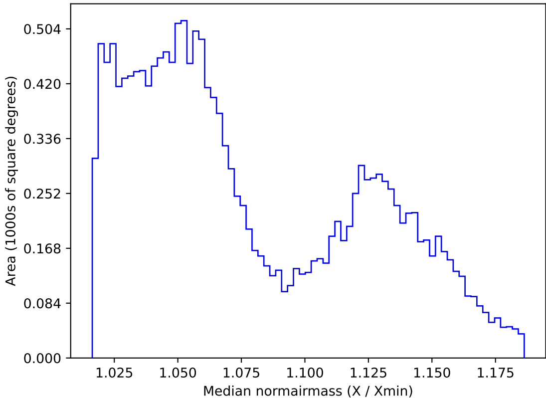
too_elab_r32_d3_griz_v3.4_10yrs WFD r band: Median normairmass
