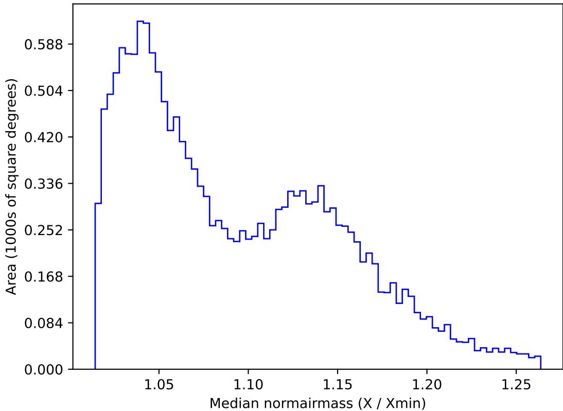
too_elab_r32_d3_griz_v3.4_10yrs WFD g band: Median normairmass
