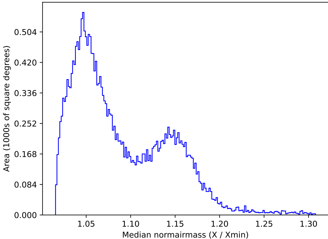
too_elab_r32_d3_griz_v3.4_10yrs All sky z band: Median normairmass
