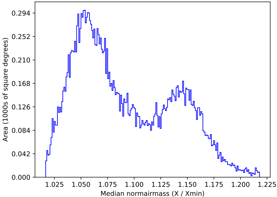
too_elab_r32_d3_griz_v3.4_10yrs All sky y band: Median normairmass
