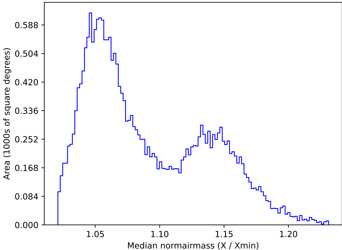
too_elab_r32_d3_griz_v3.4_10yrs All sky y band: Median normairmass
