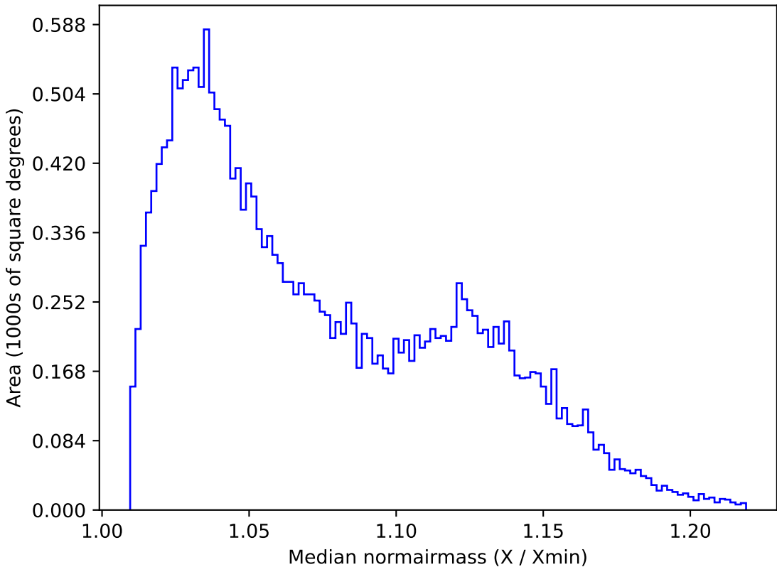
too_elab_r32_d3_griz_v3.4_10yrs All sky u band: Median normairmass
