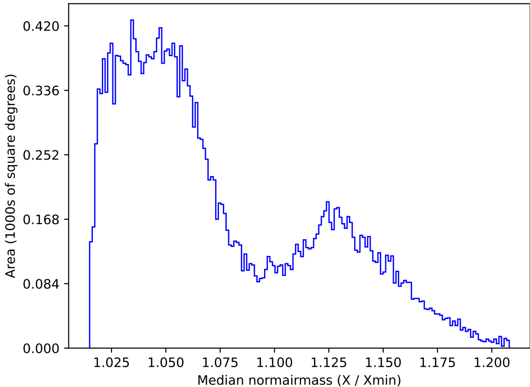
too_elab_r32_d3_griz_v3.4_10yrs All sky r band: Median normairmass
