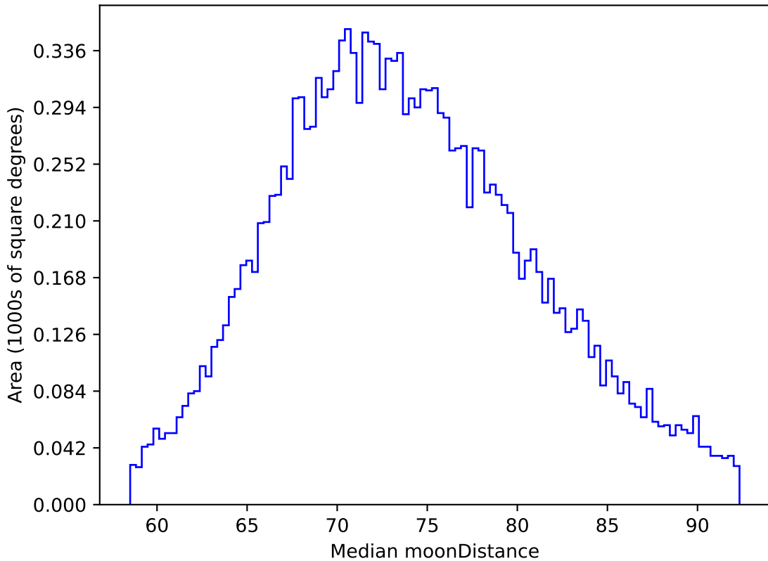
too_elab_r32_d3_griz_v3.4_10yrs WFD z band: Median moonDistance
