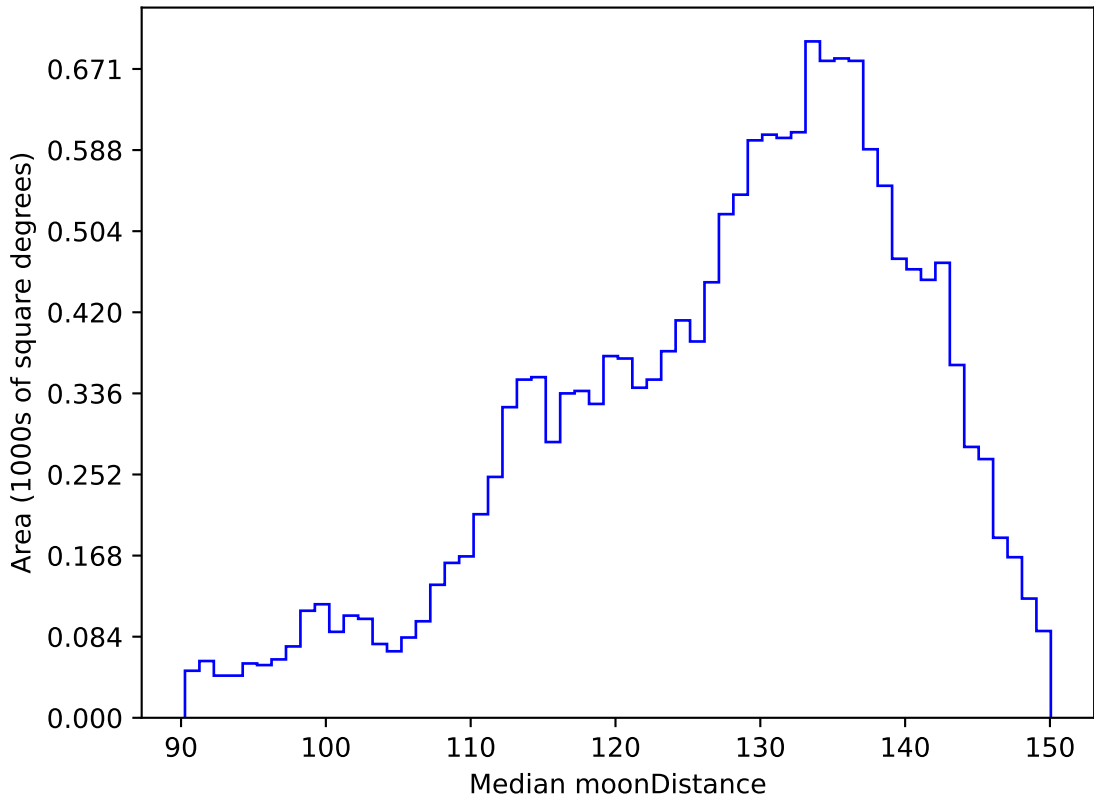
too_elab_r32_d3_griz_v3.4_10yrs WFD u band: Median moonDistance
