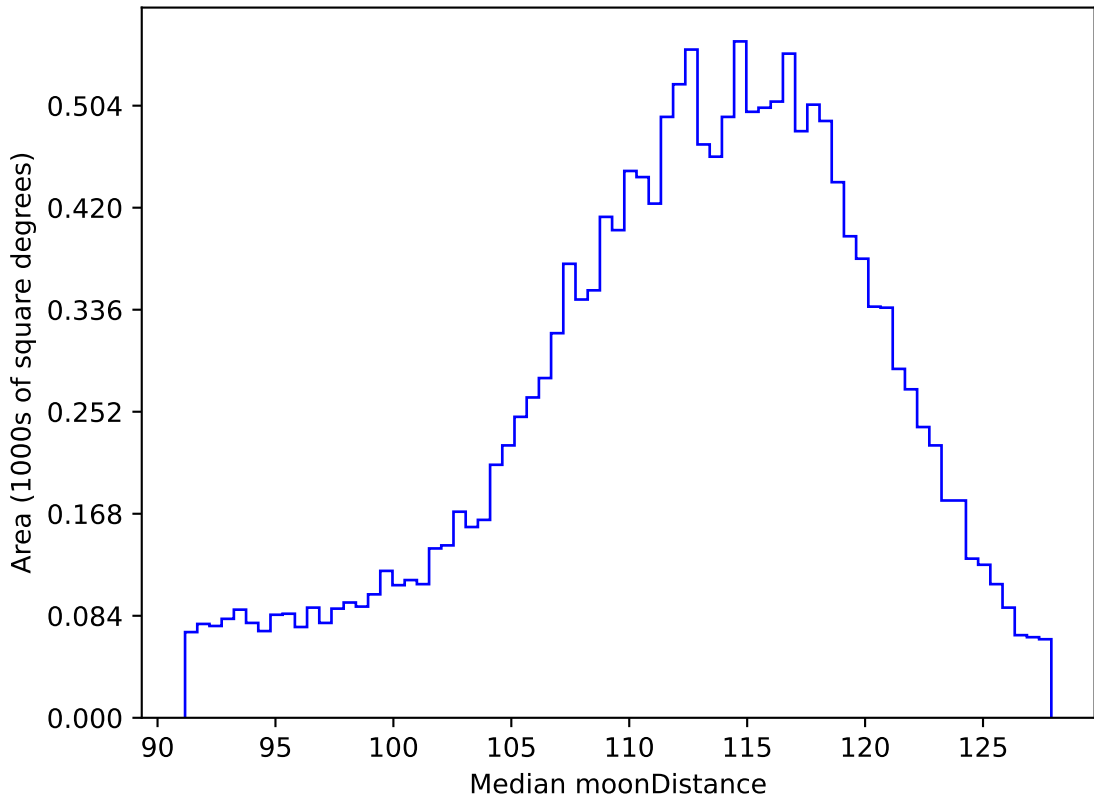
too_elab_r32_d3_griz_v3.4_10yrs WFD r band: Median moonDistance
