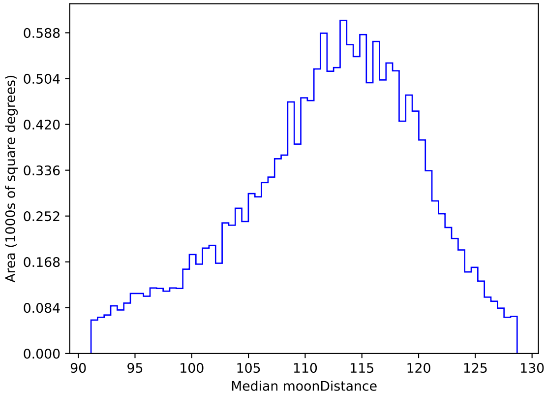
too_elab_r32_d3_griz_v3.4_10yrs WFD r band: Median moonDistance
