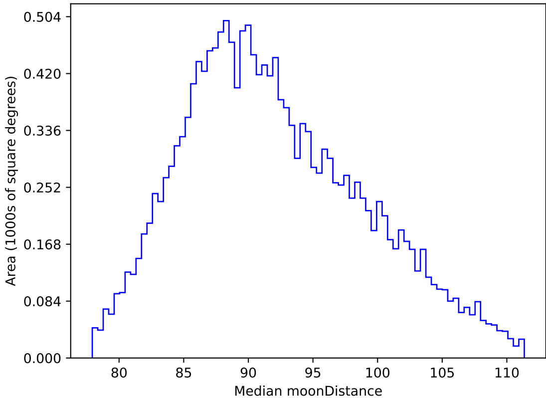
too_elab_r32_d3_griz_v3.4_10yrs WFD i band: Median moonDistance
