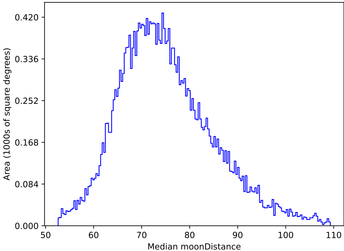
too_elab_r32_d3_griz_v3.4_10yrs All sky z band: Median moonDistance
