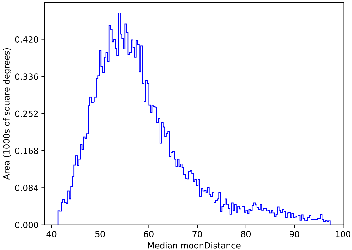
too_elab_r32_d3_griz_v3.4_10yrs All sky y band: Median moonDistance
