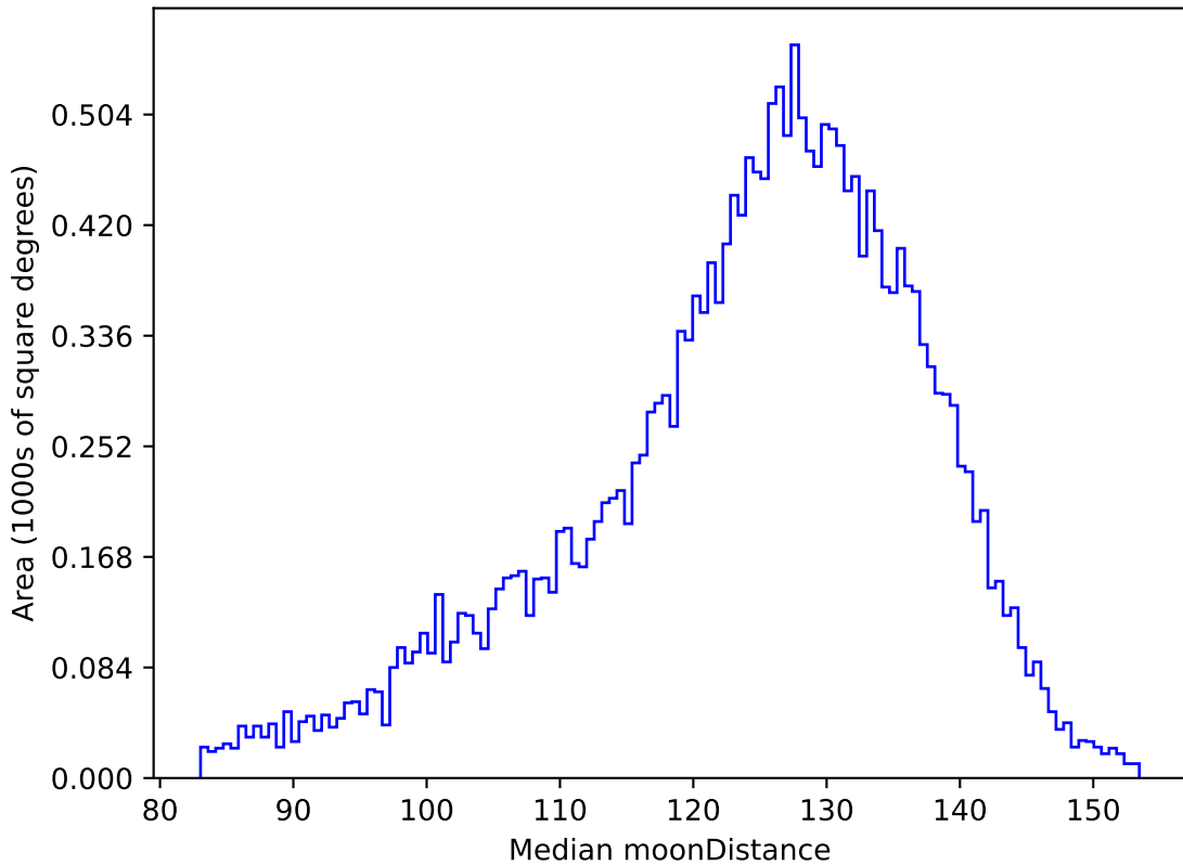
too_elab_r32_d3_griz_v3.4_10yrs All sky u band: Median moonDistance
