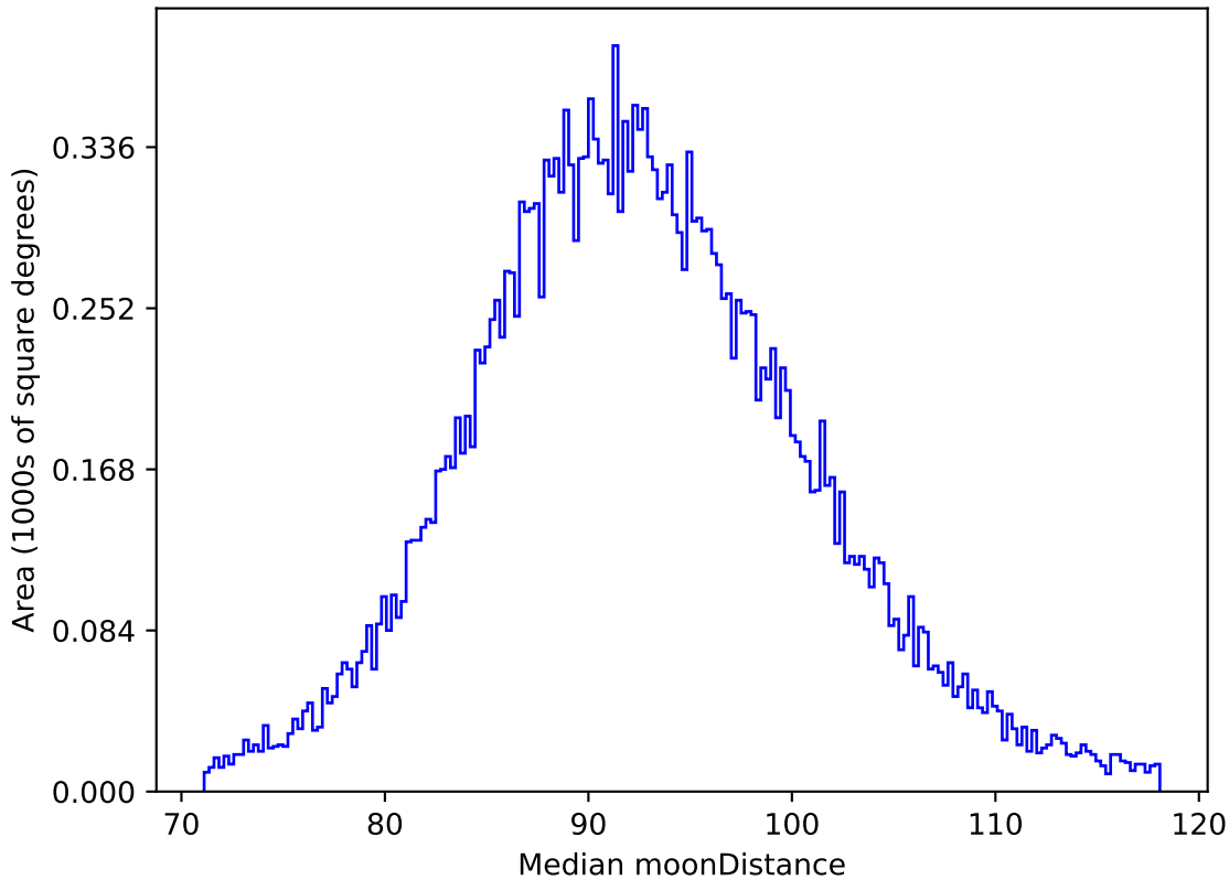
too_elab_r32_d3_griz_v3.4_10yrs All sky i band: Median moonDistance
