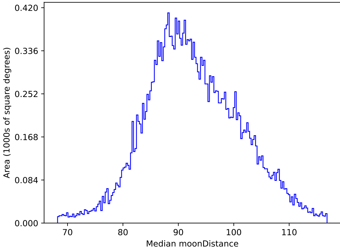
too_elab_r32_d3_griz_v3.4_10yrs All sky i band: Median moonDistance
