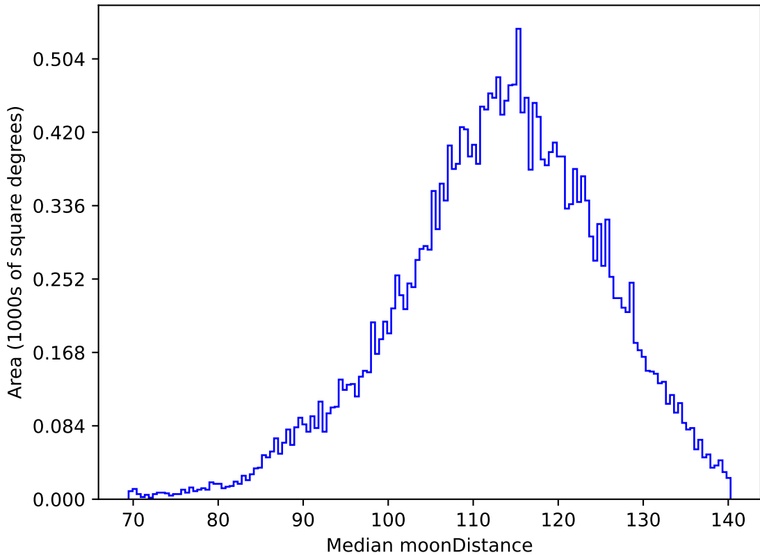
too_elab_r32_d3_griz_v3.4_10yrs All sky g band: Median moonDistance
