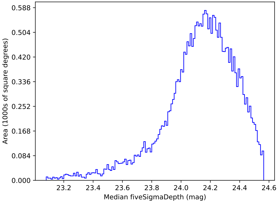
too_elab_r32_d3_griz_v3.4_10yrs Yr 1 r band: Median fiveSigmaDepth
