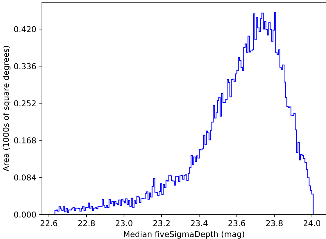
too_elab_r32_d3_griz_v3.4_10yrs Yr 1 i band: Median fiveSigmaDepth
