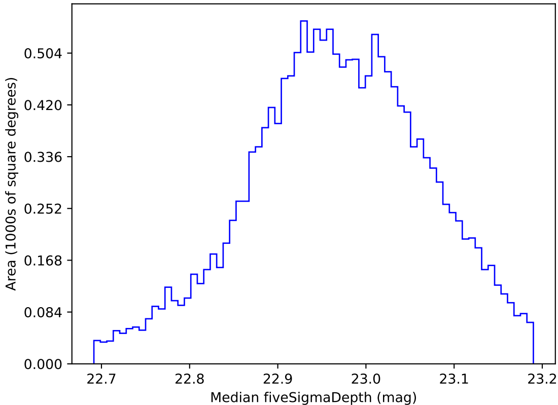
too_elab_r32_d3_griz_v3.4_10yrs WFD z band: Median fiveSigmaDepth
