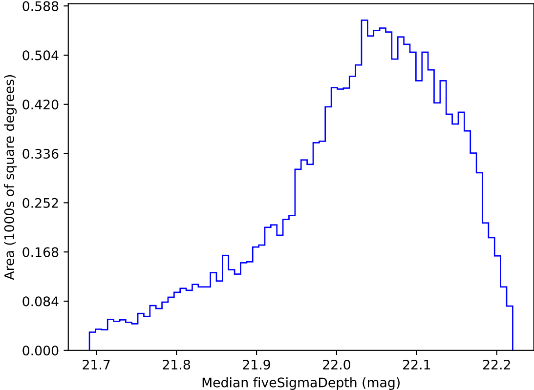
too_elab_r32_d3_griz_v3.4_10yrs WFD y band: Median fiveSigmaDepth
