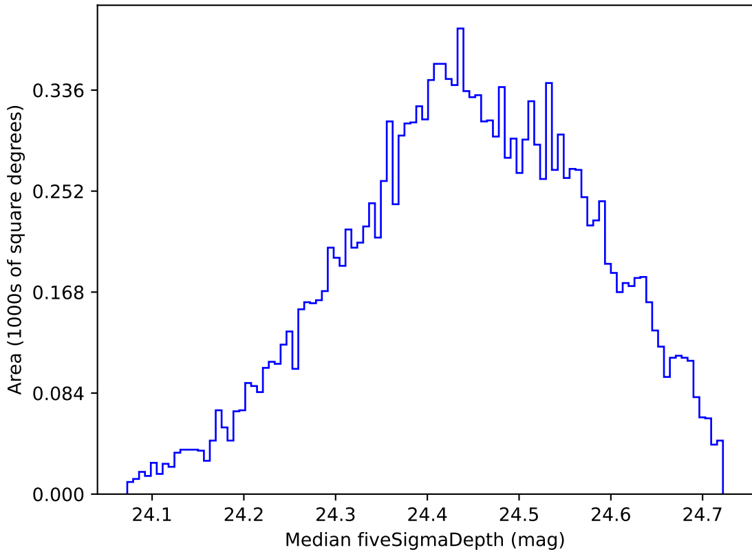
too_elab_r32_d3_griz_v3.4_10yrs WFD g band: Median fiveSigmaDepth
