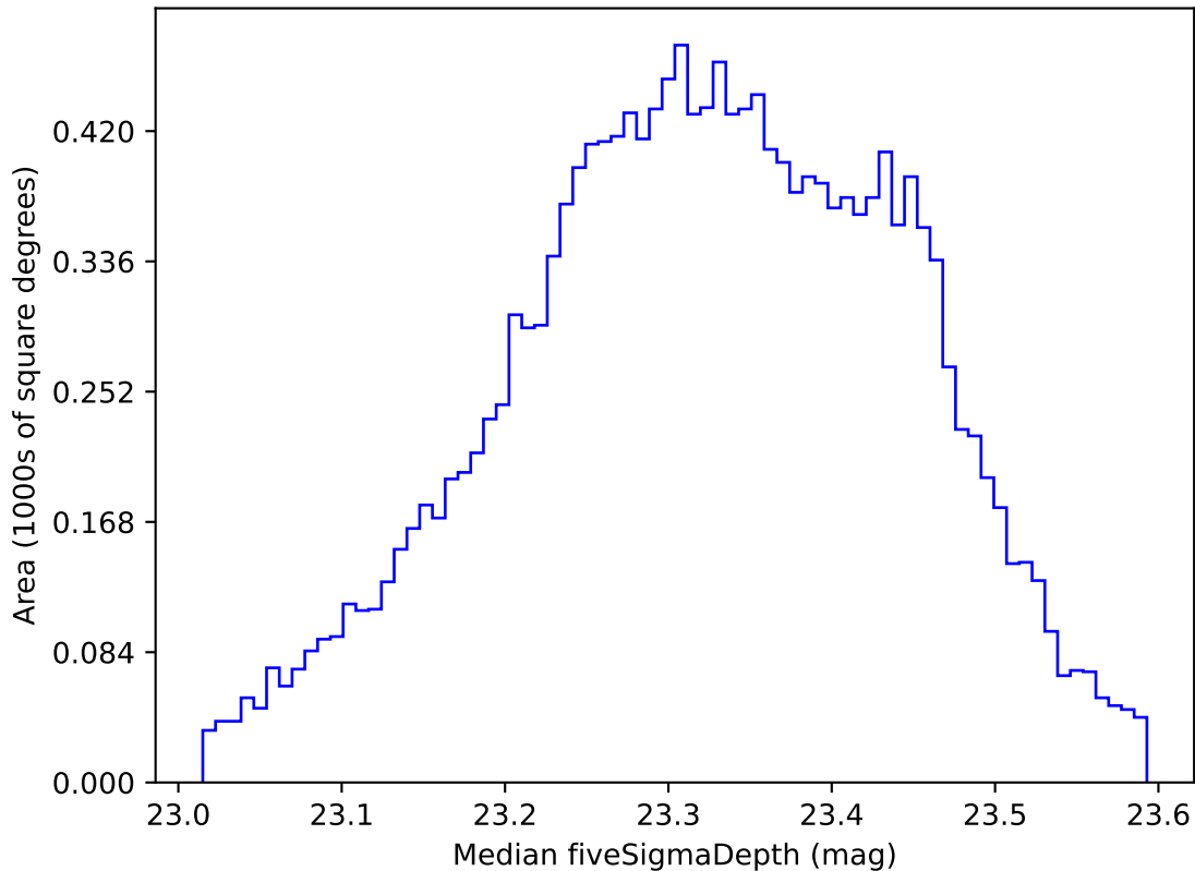
too_elab_r32_d3_griz_v3.4_10yrs WFD all bands: Median fiveSigmaDepth
