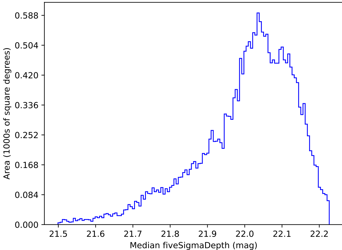
too_elab_r32_d3_griz_v3.4_10yrs All sky y band: Median fiveSigmaDepth
