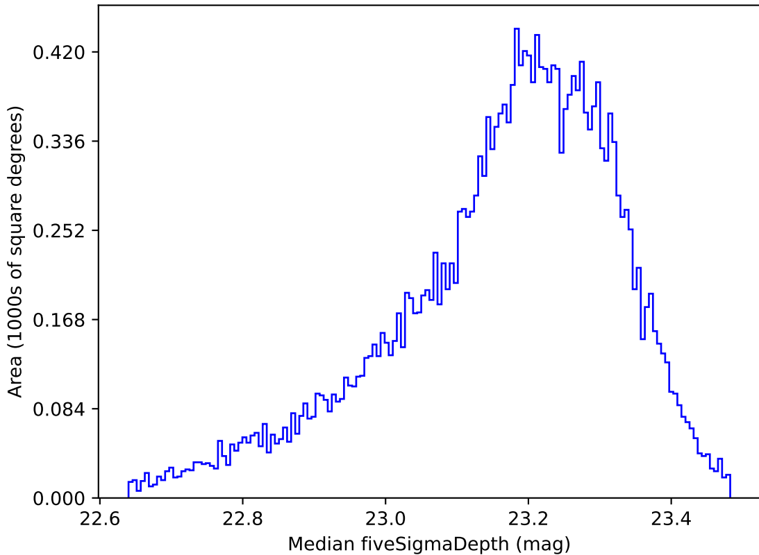
too_elab_r32_d3_griz_v3.4_10yrs All sky u band: Median fiveSigmaDepth
