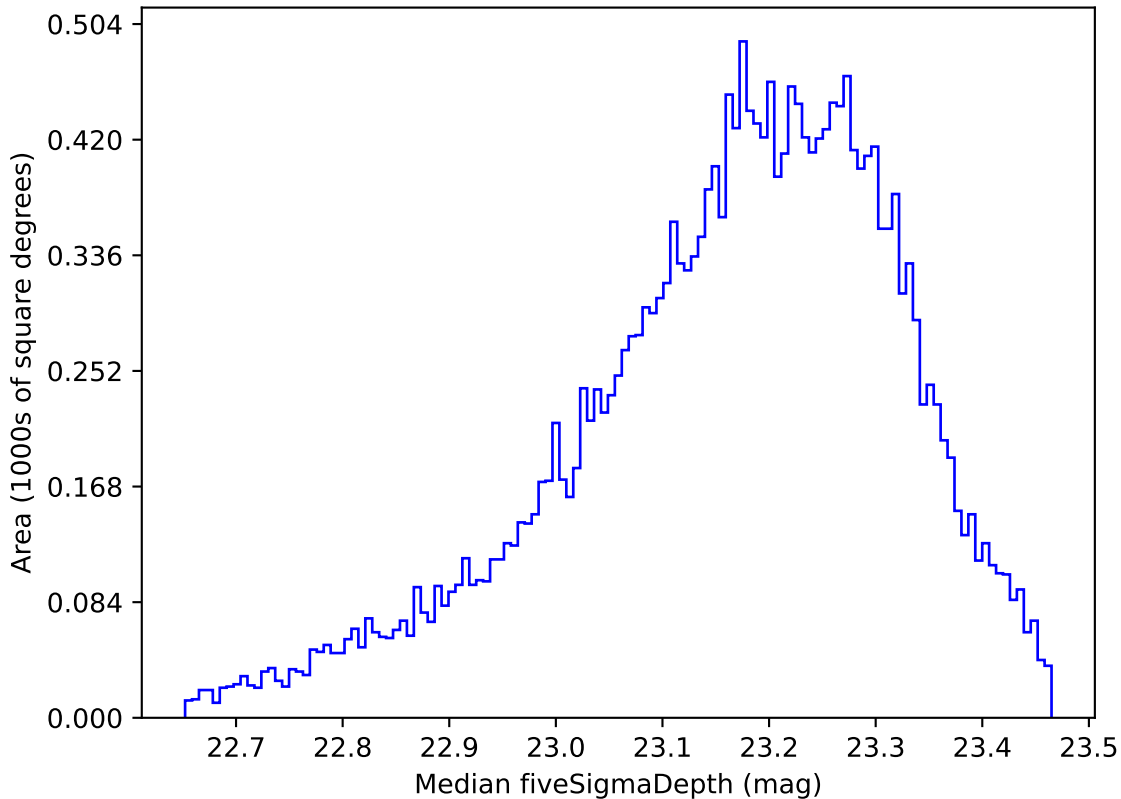
too_elab_r32_d3_griz_v3.4_10yrs All sky u band: Median fiveSigmaDepth
