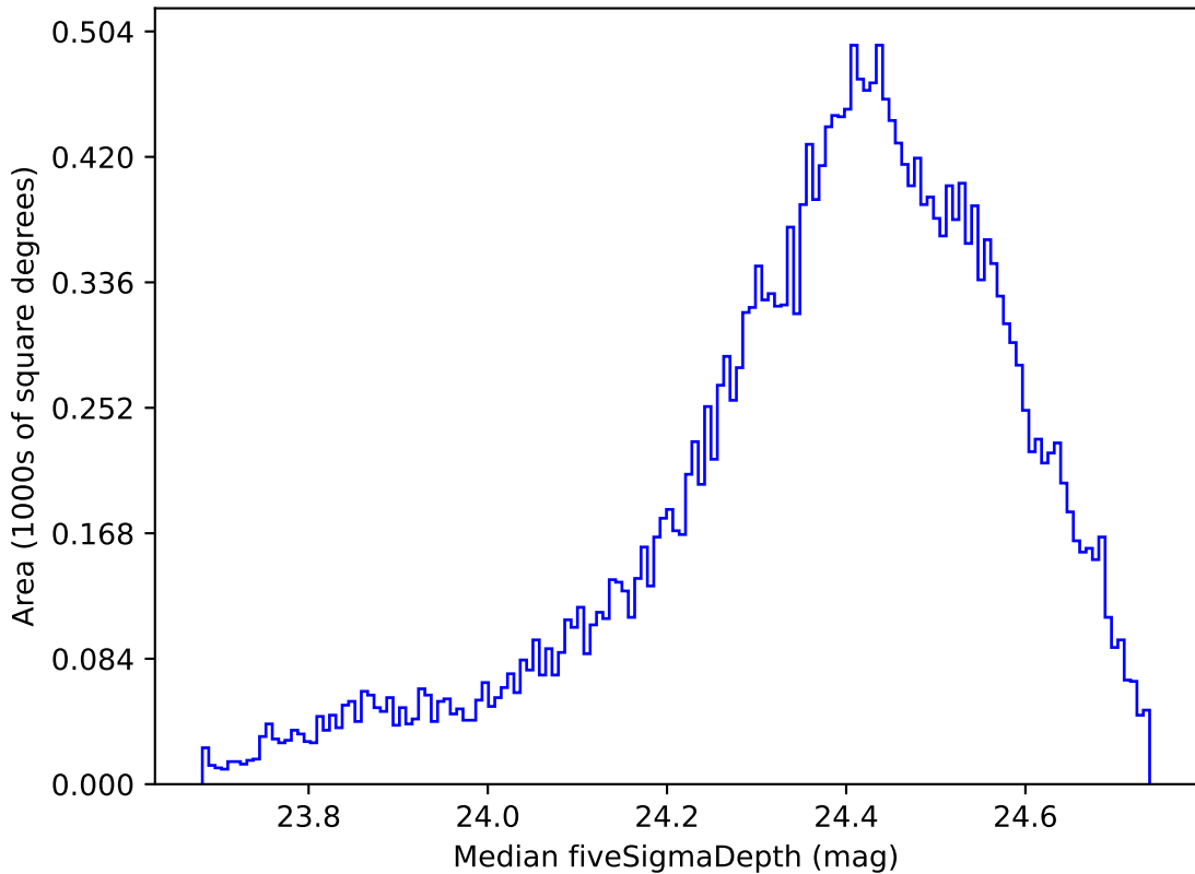
too_elab_r32_d3_griz_v3.4_10yrs All sky g band: Median fiveSigmaDepth
