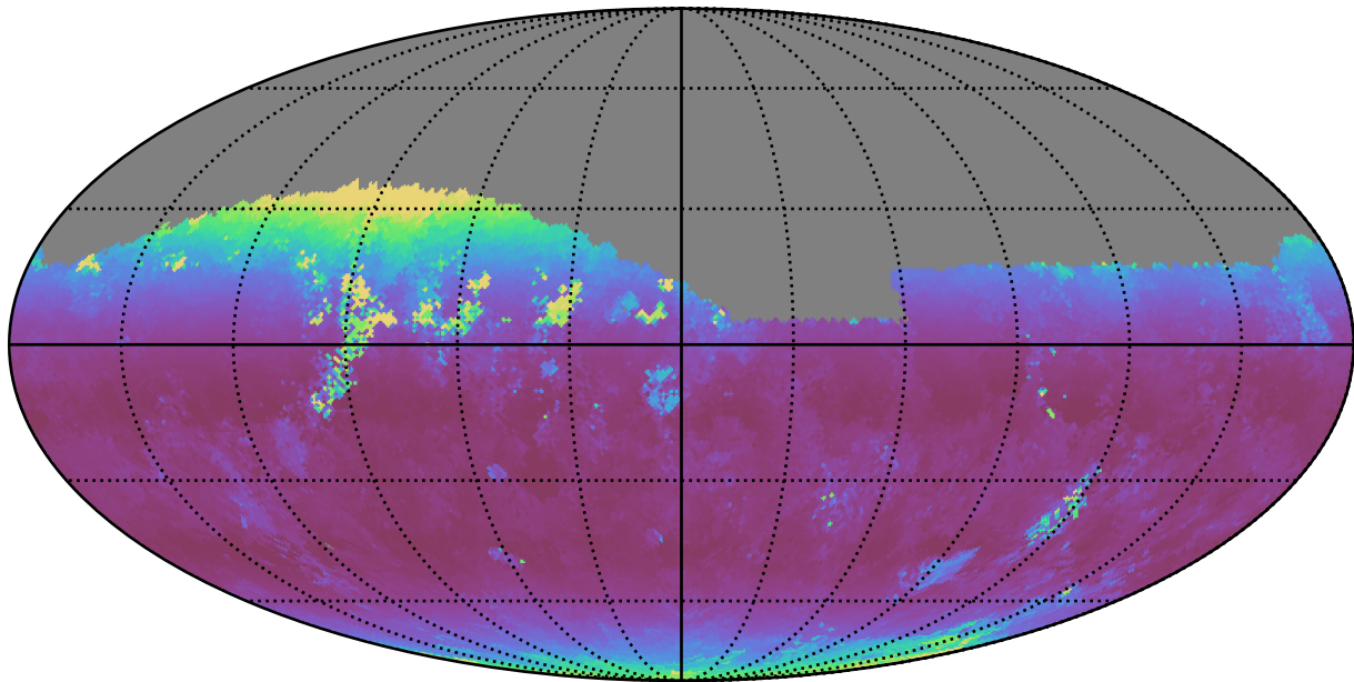
too_elab_r32_d3_griz_v3.4_10yrs Yr 1 z band: Median airmass
