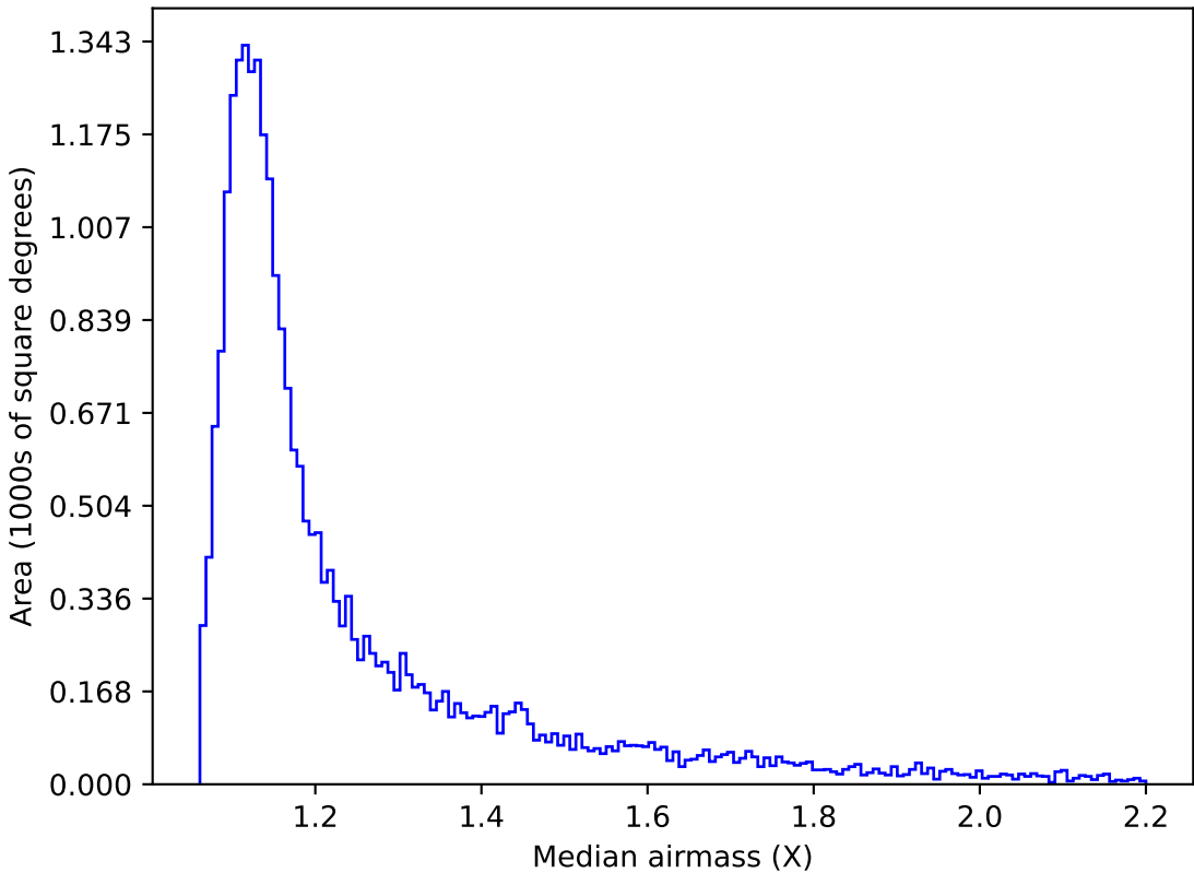
too_elab_r32_d3_griz_v3.4_10yrs Yr 1 z band: Median airmass
