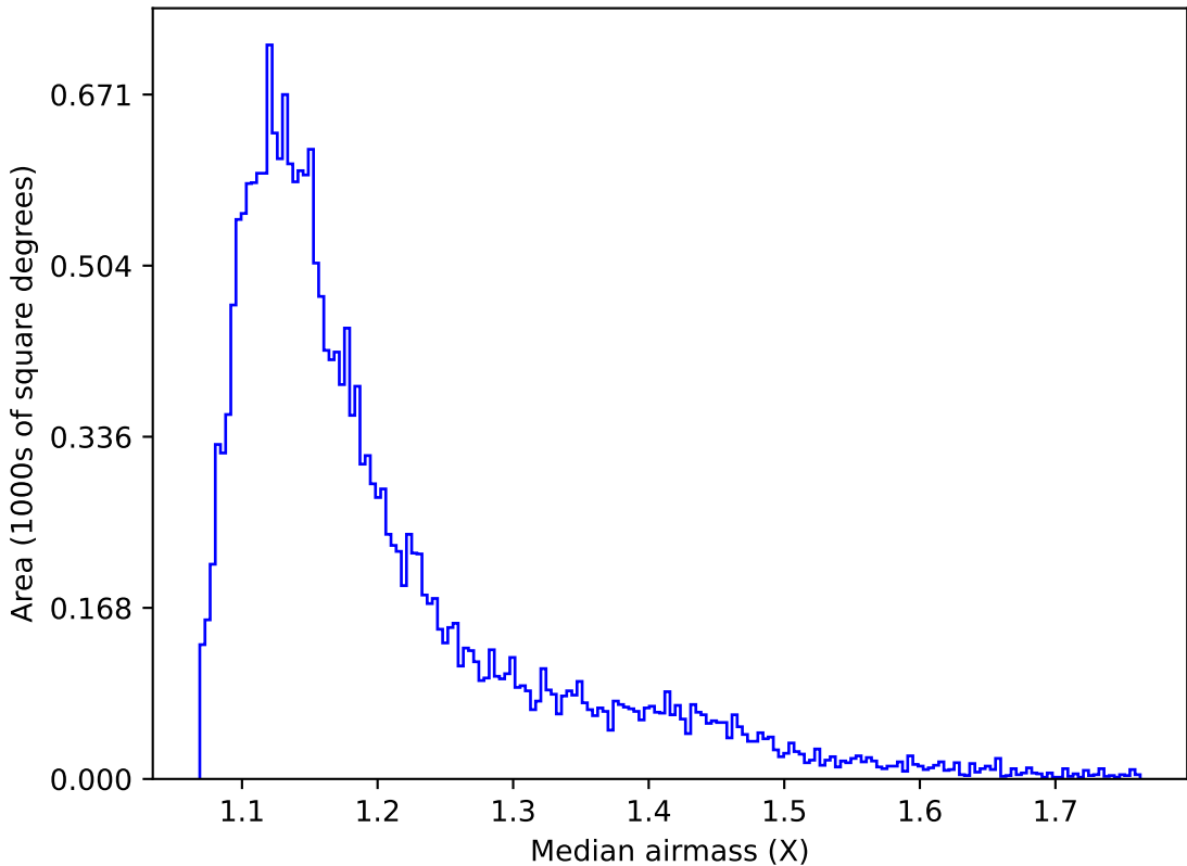
too_elab_r32_d3_griz_v3.4_10yrs Yr 1 y band: Median airmass
