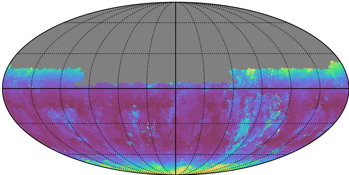
too_elab_r32_d3_griz_v3.4_10yrs Yr 1 u band: Median airmass
