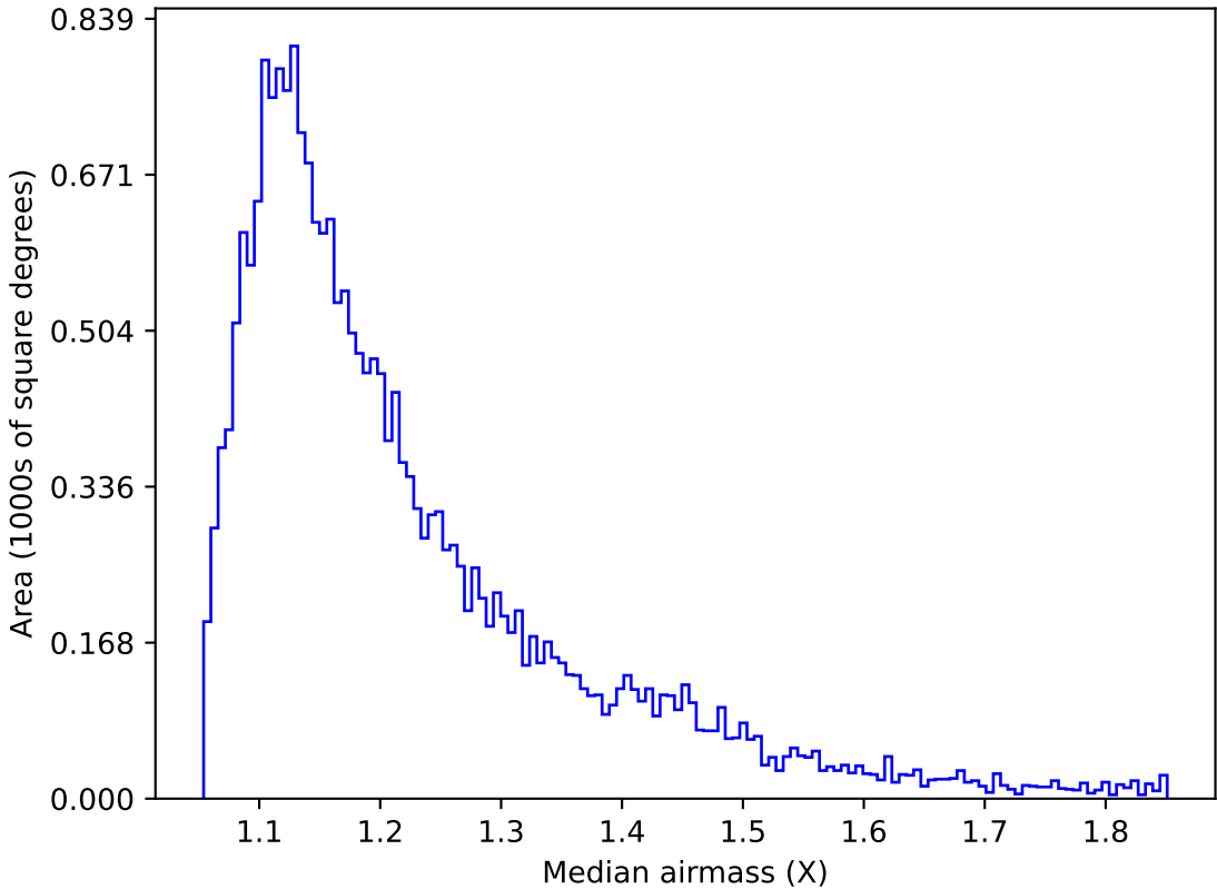
too_elab_r32_d3_griz_v3.4_10yrs Yr 1 u band: Median airmass
