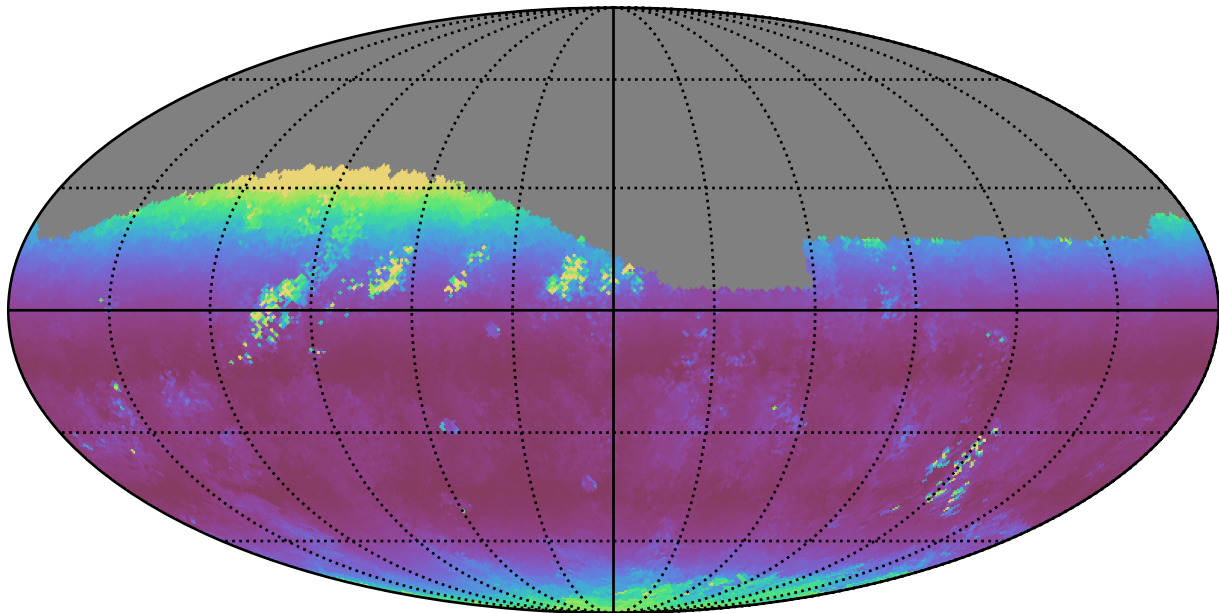
too_elab_r32_d3_griz_v3.4_10yrs Yr 1 r band: Median airmass
