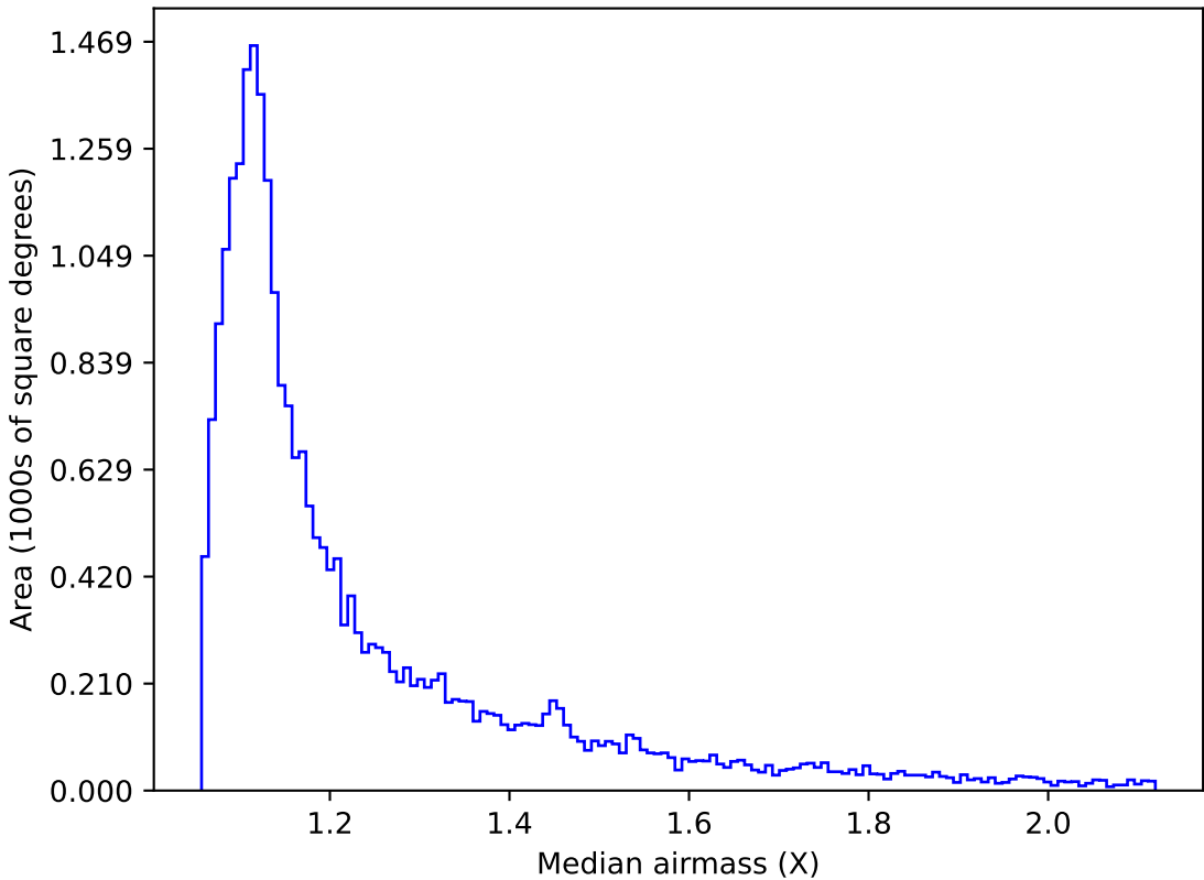
too_elab_r32_d3_griz_v3.4_10yrs Yr 1 r band: Median airmass
