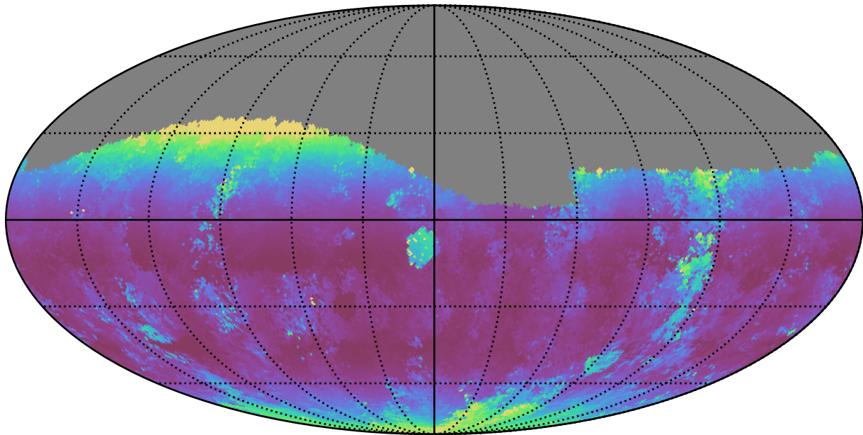
too_elab_r32_d3_griz_v3.4_10yrs Yr 1 g band: Median airmass
