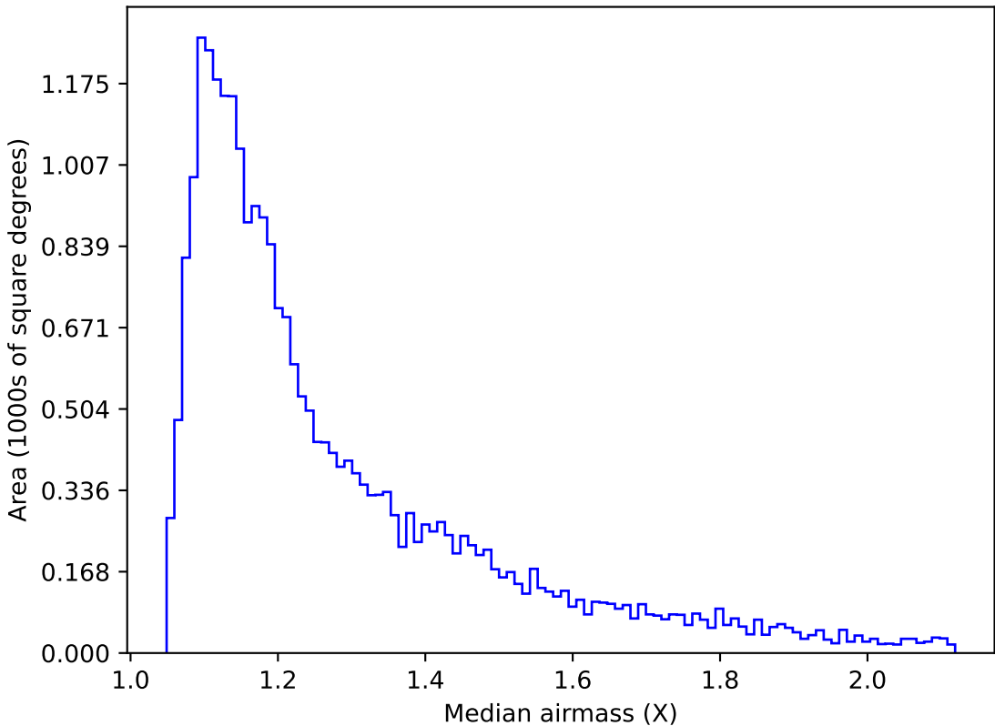
too_elab_r32_d3_griz_v3.4_10yrs Yr 1 g band: Median airmass
