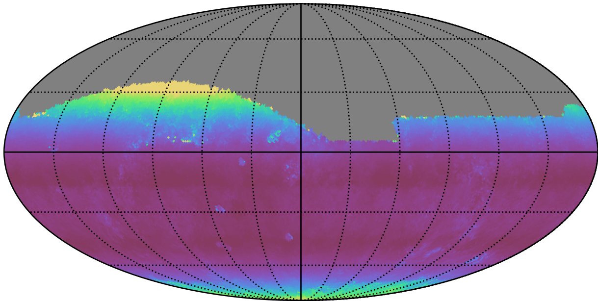
too_elab_r32_d3_griz_v3.4_10yrs Yr 1 all bands: Median airmass
