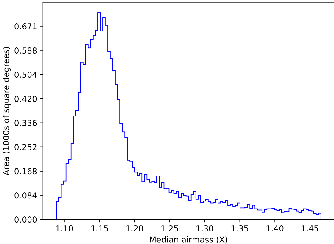
too_elab_r32_d3_griz_v3.4_10yrs WFD z band: Median airmass
