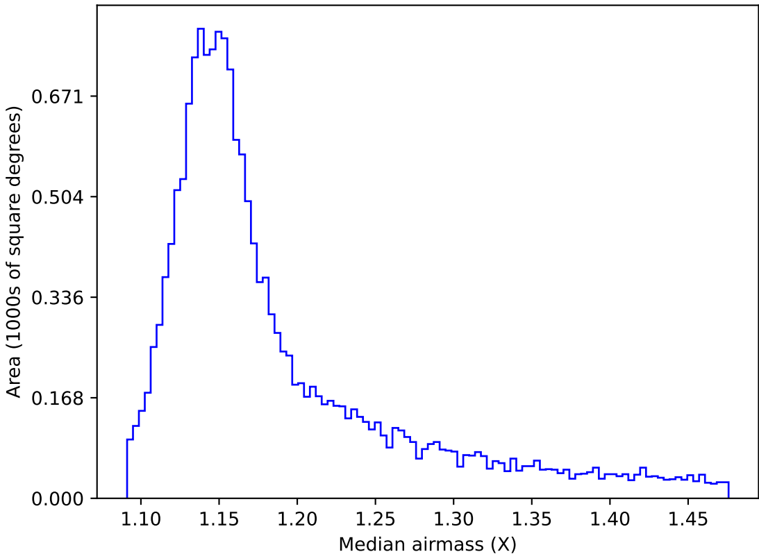
too_elab_r32_d3_griz_v3.4_10yrs WFD y band: Median airmass
