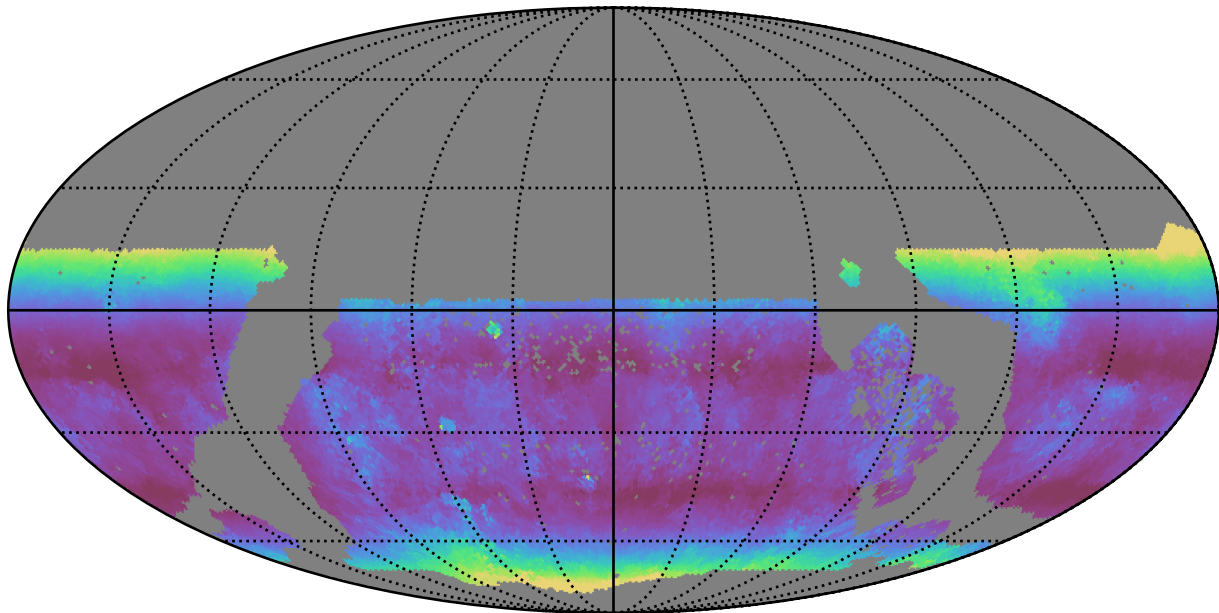
too_elab_r32_d3_griz_v3.4_10yrs WFD u band: Median airmass
