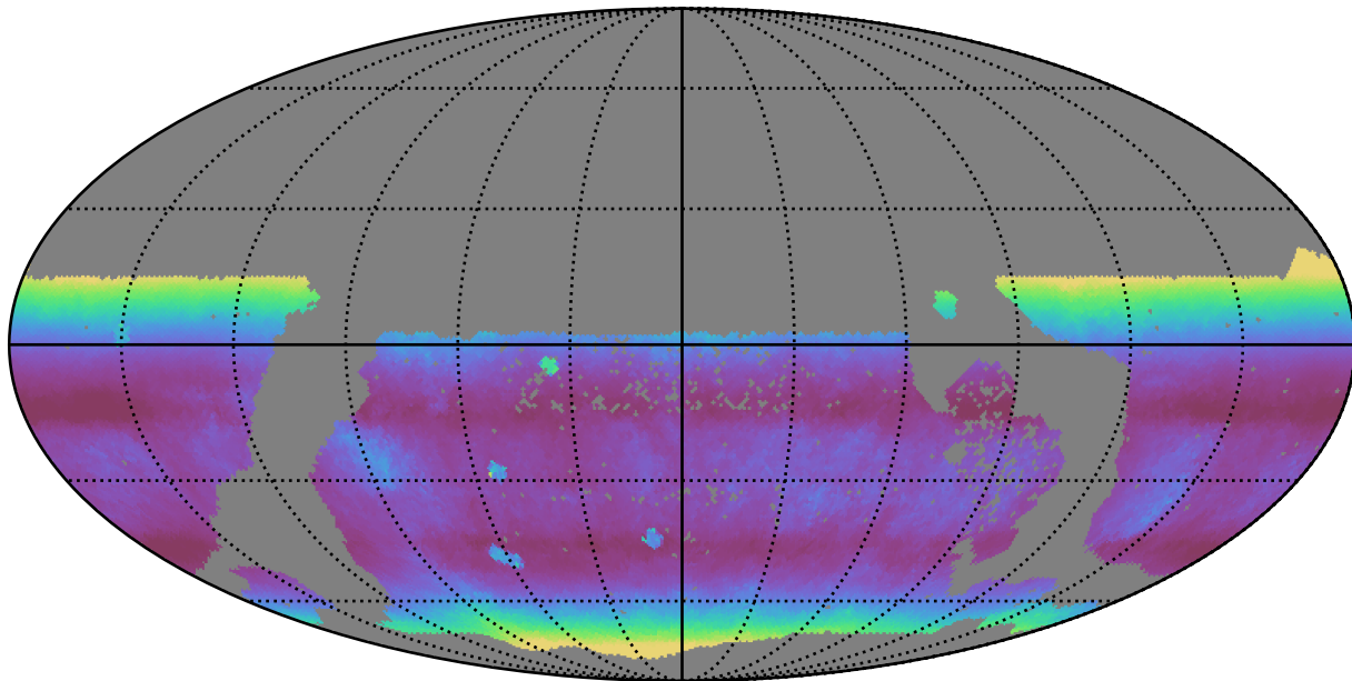
too_elab_r32_d3_griz_v3.4_10yrs WFD r band: Median airmass
