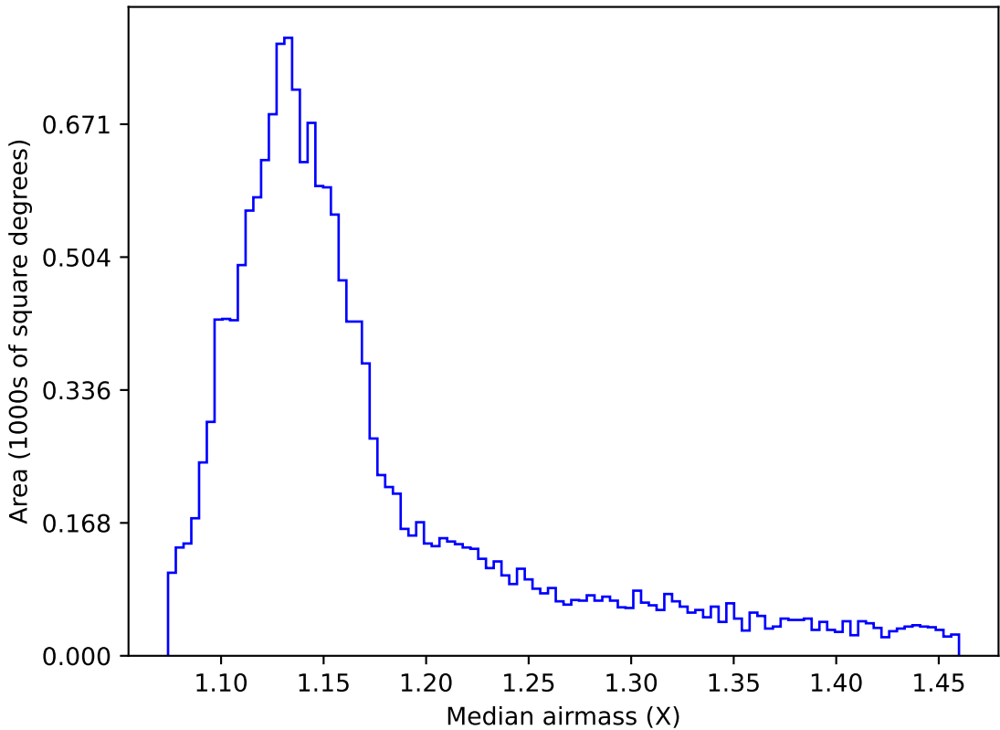
too_elab_r32_d3_griz_v3.4_10yrs WFD r band: Median airmass
