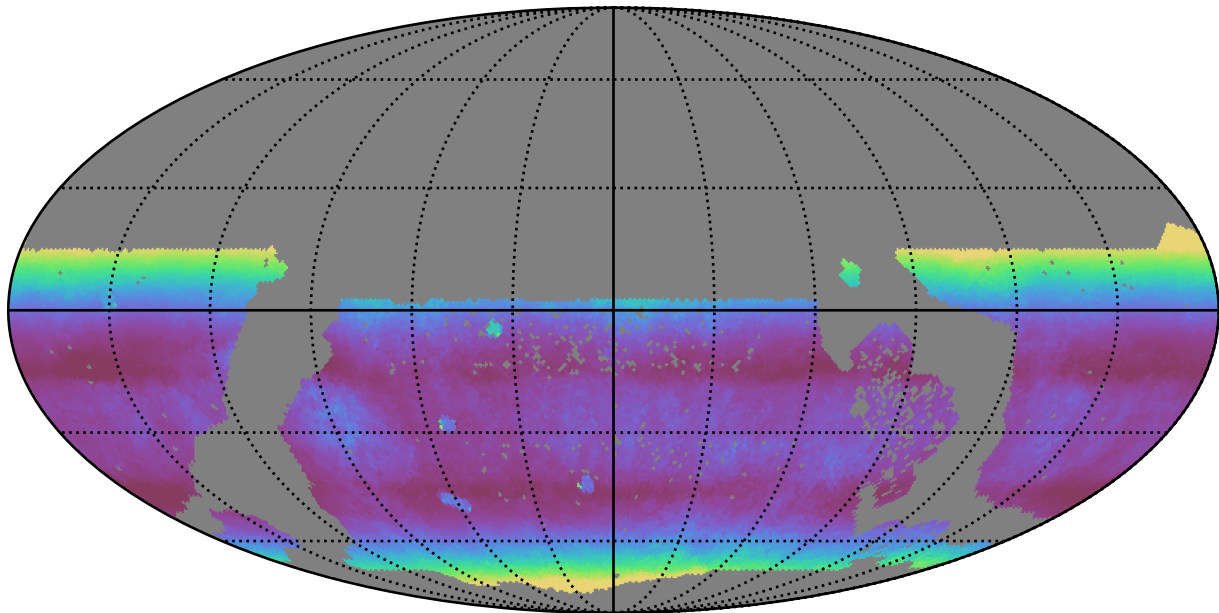
too_elab_r32_d3_griz_v3.4_10yrs WFD i band: Median airmass
