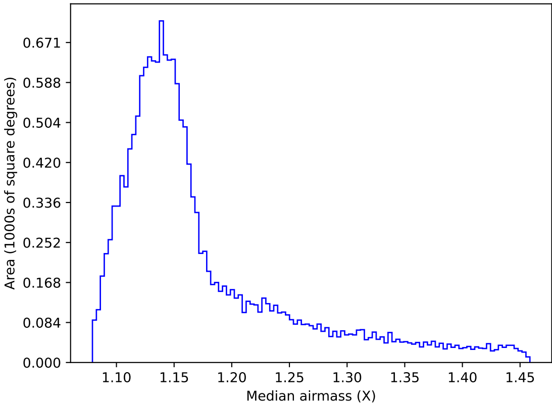
too_elab_r32_d3_griz_v3.4_10yrs WFD i band: Median airmass
